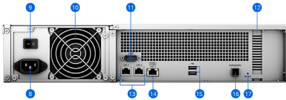
RS2423+ (后面板)
