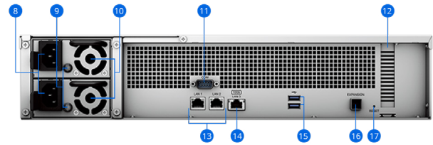
RS2423RP+ (后面板)
